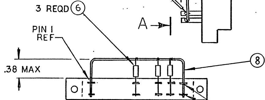
VIEW A-A ROTATED CCW 90° WIRES NOT SHOWN FOR CLARITY
